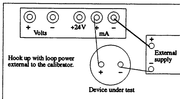
Figure 1. Loop power is supplied by a power supply in the loop. The calibrator is hooked in series with the remainder of the loop where applicable.
