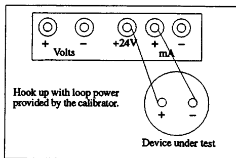
Figure 2. The PneuCal IV-B supplies power to the loop. The calibrator is hooked in series with the remainder of the loop where applicable. Use this hookup to test pressure switches.
