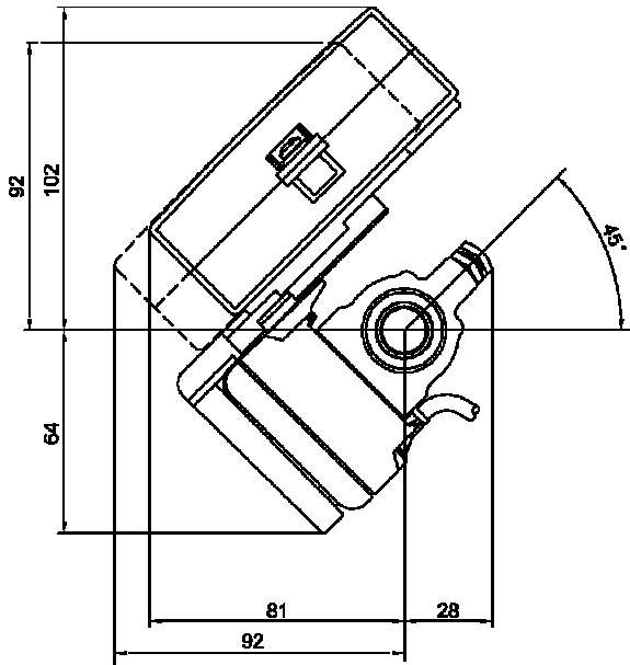
MULTICAL® 601 mounted on ULTRAFLOW®
